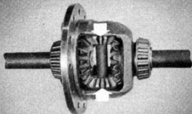
DIFFERENTIAL PINIONS (FREE TO ROTATE ON SHAFT)
